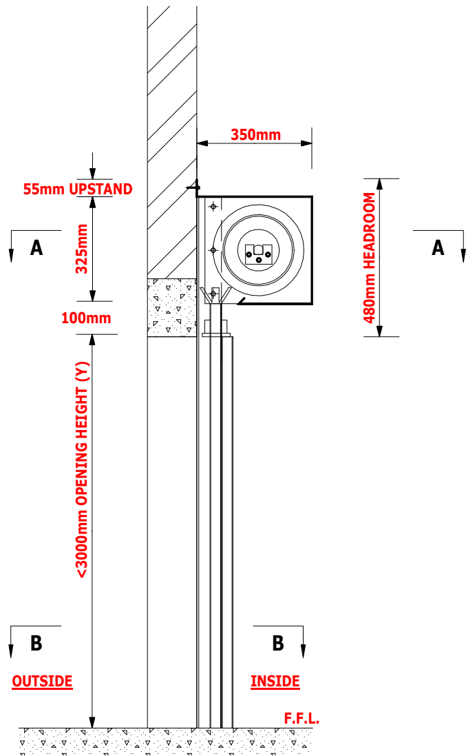
SECTION C-C
